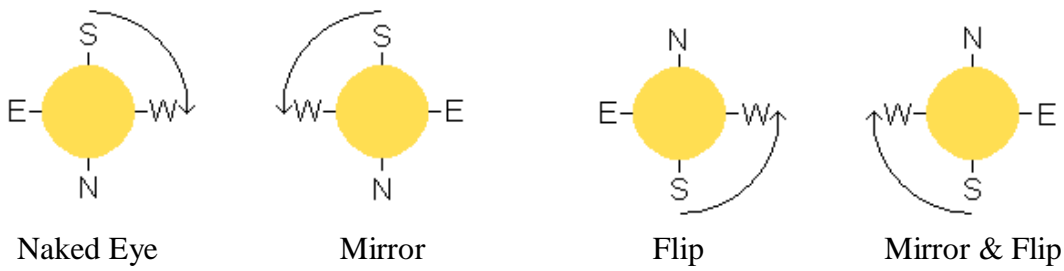
Figure 4b. The naked eye orientation of the Sun (left) for a southern hemisphere observer and when on the meridian together with mirrored and/or flipped orientations. The arrow indicates the rotation direction for a positive values of \eta or T .
