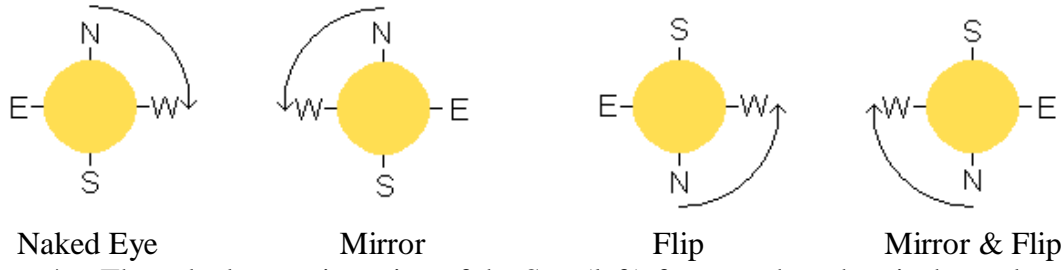
Figure 4a. The naked eye orientation of the Sun (left) for a northern hemisphere observer and when on the meridian together with mirrored and/or flipped orientations. The arrow indicates the rotation direction for a positive values of \eta or T .
